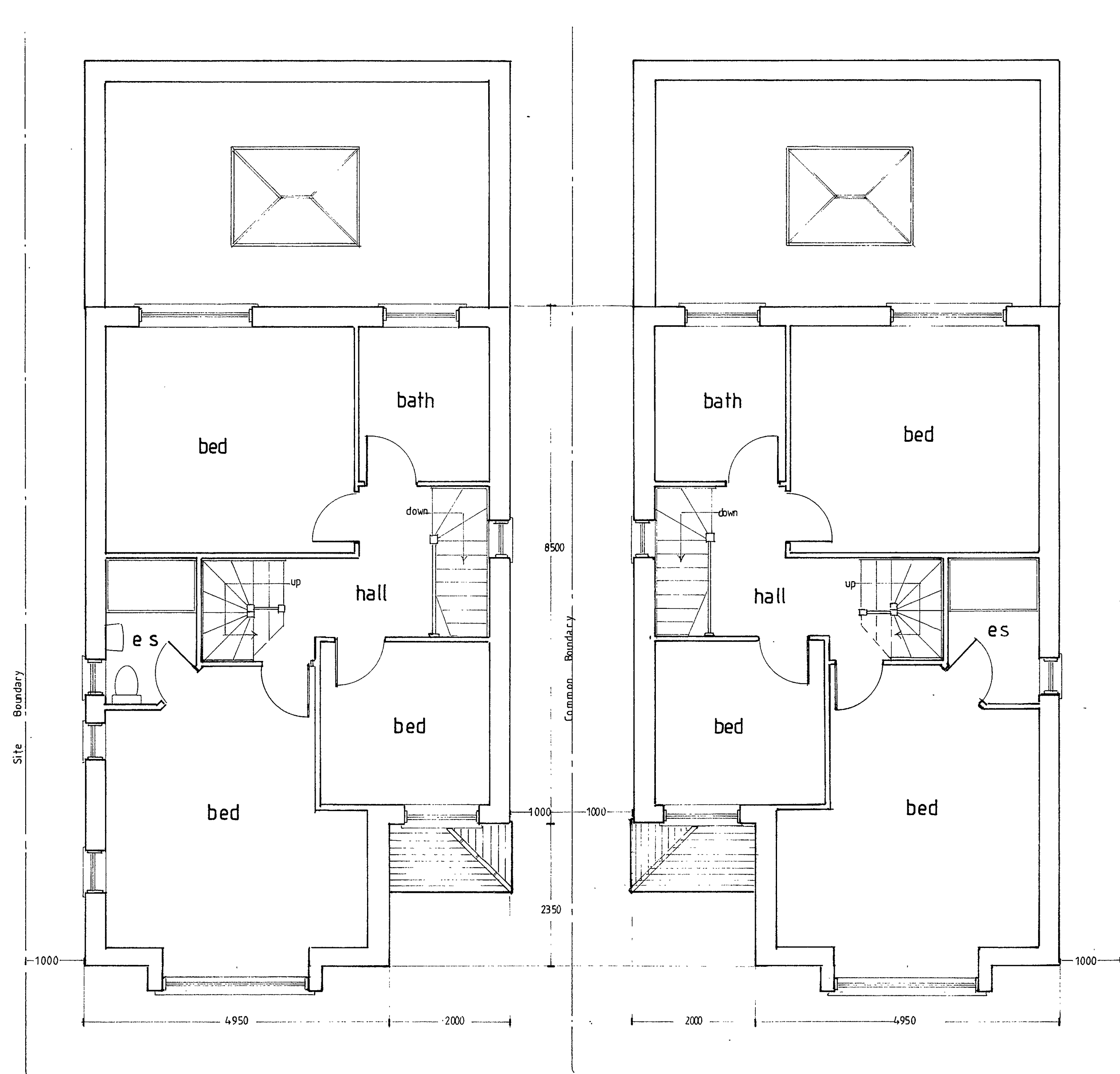
Proposed First Floor Plan 1:50.
